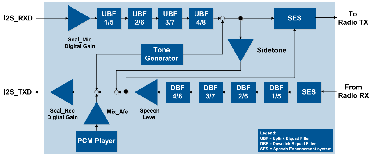
Figure 18: Audio paths
