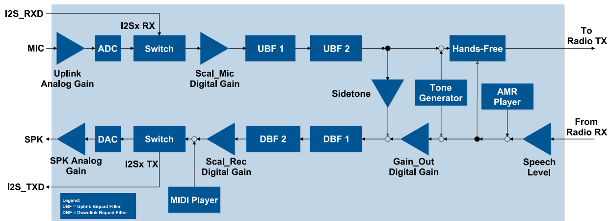
Figure 21: Audio paths
