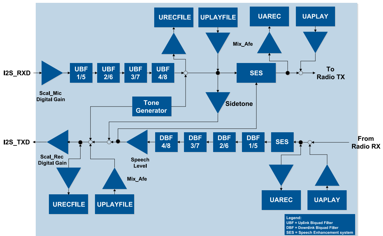
Figure 17: Audio paths of SARA-U201 / SARA-U270 "04" product versions
