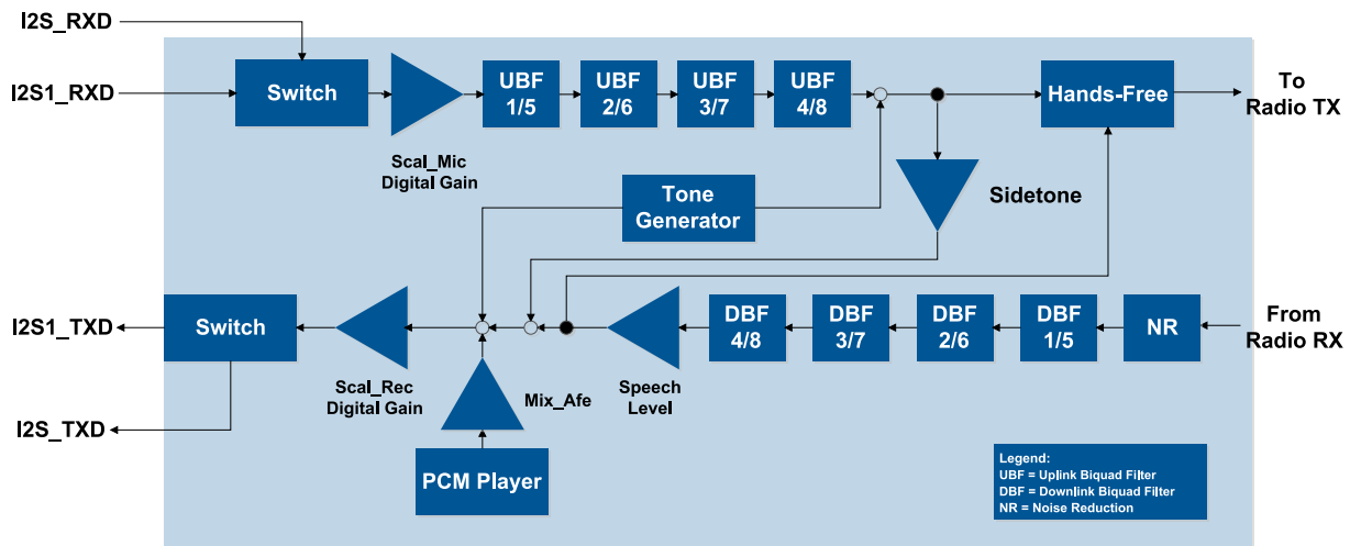
Figure 19: Audio paths
