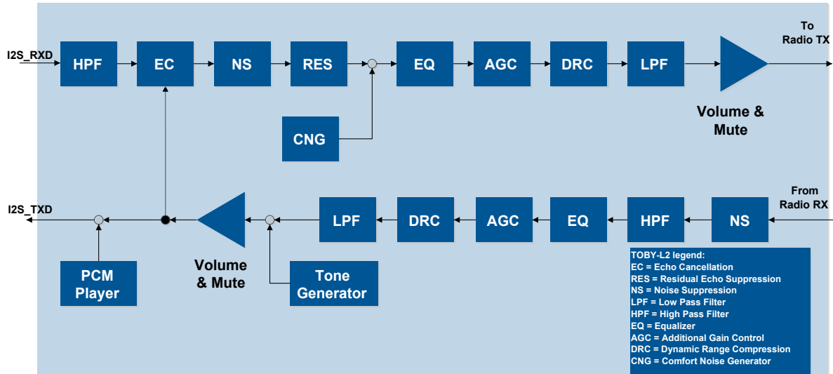
Figure 13: Audio paths
