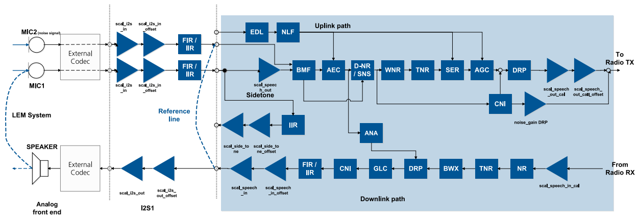
Figure 15: Audio digital path
