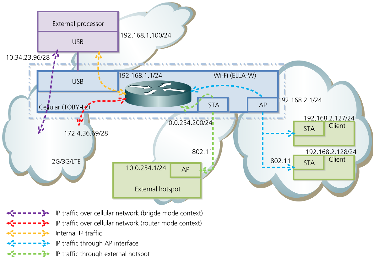
Figure 27: Bridge mode with Internet access via cellular network or via external hotspot
