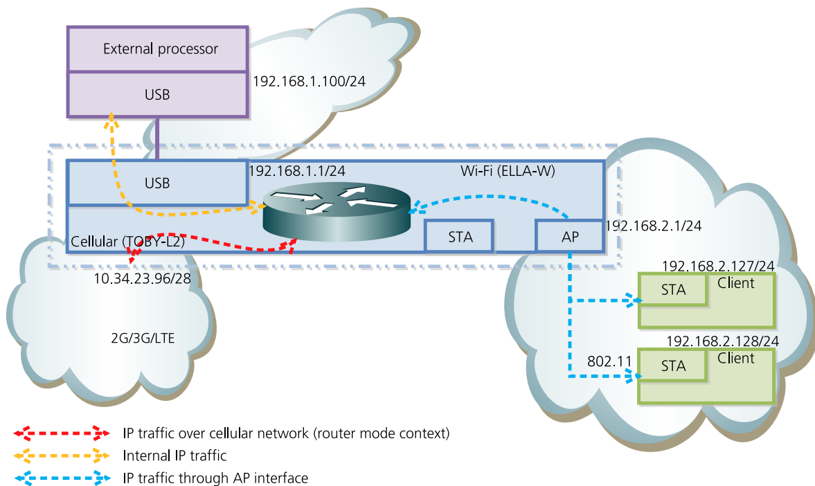
Figure 21: Router mode with Internet access via cellular network
