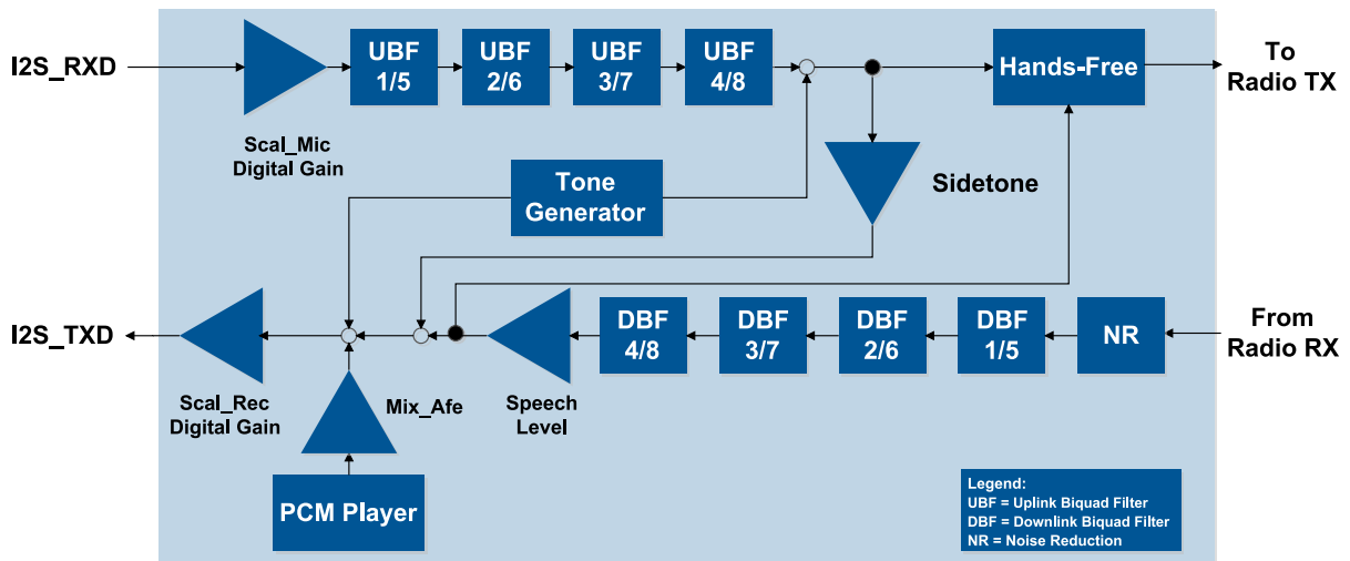
Figure 14: Audio paths
