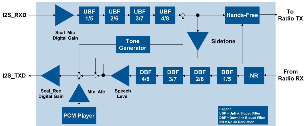
Figure 15: Audio paths
