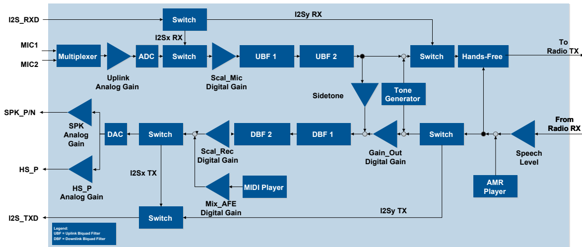
Figure 19: Audio paths
