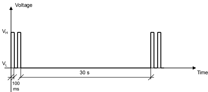
Figure 10: GPIO pin progress for registered roaming 4G Cat M1
