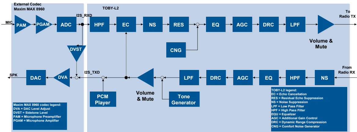
Figure 20: External codec controls
