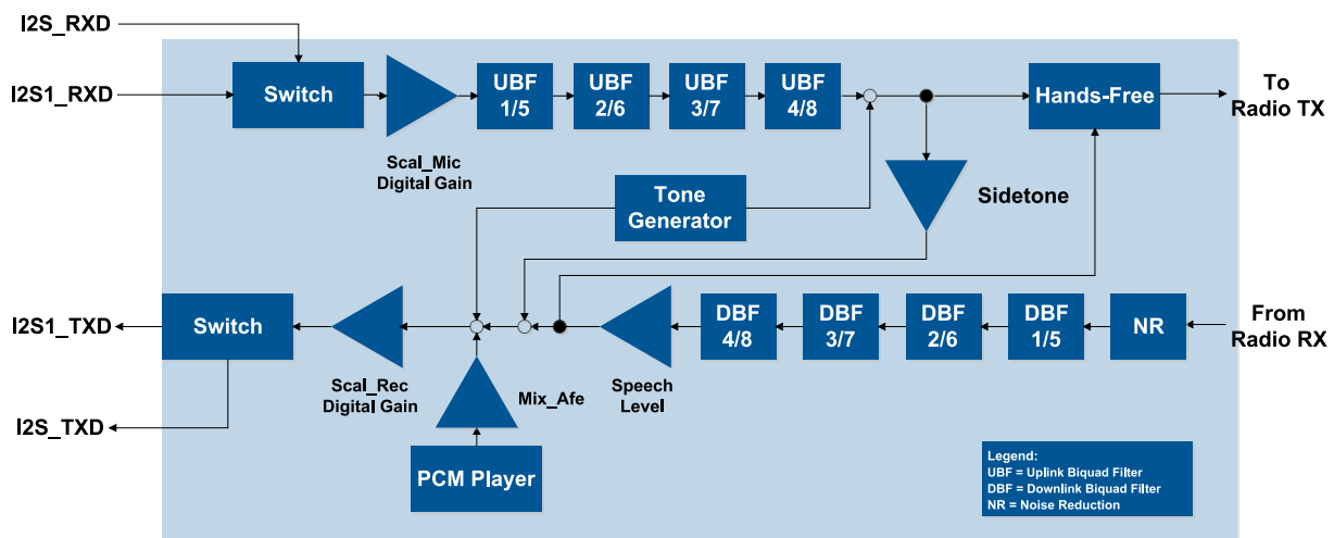
Figure 16: Audio paths
