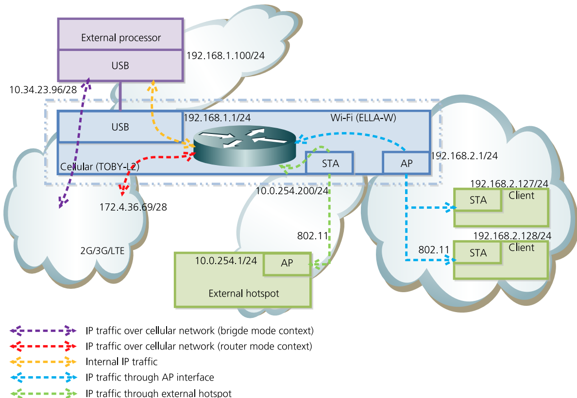
Figure 24: Bridge mode with Internet access via cellular network or via external hotspot
