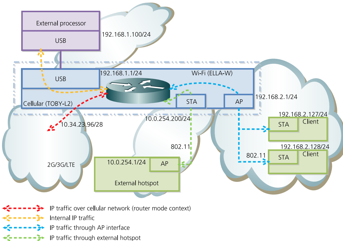
Figure 23: Router mode with Internet access via cellular network or via external hotspot
