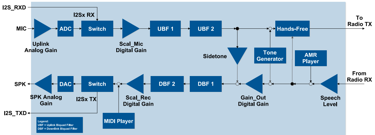
Figure 18: Audio paths
