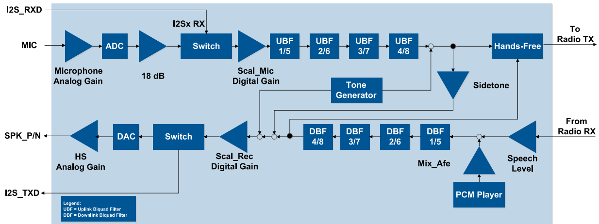
Figure 17: Audio paths
