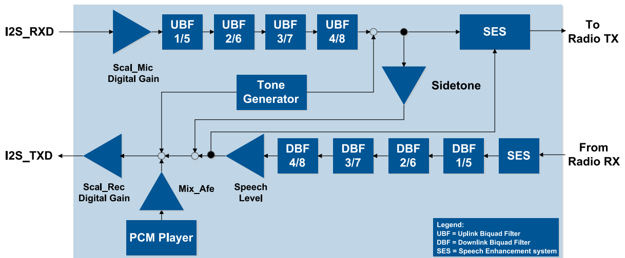
Figure 16: Audio paths
